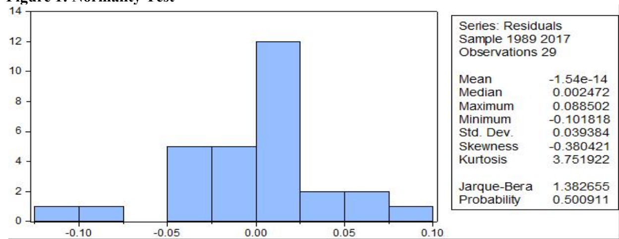
Figure 1: Normality Test
